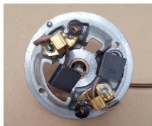
IR1113 Brush End Cover
