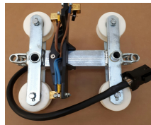
IR1006 Trolley Assembly
